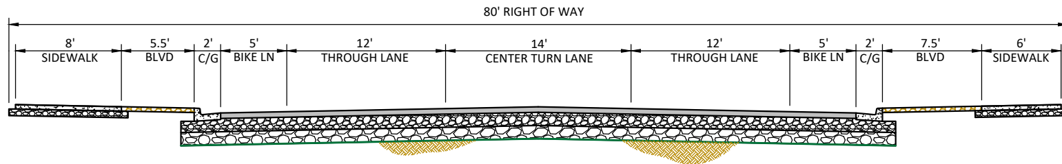
ULTIMATE ROAD SECTION (FUTURE)
