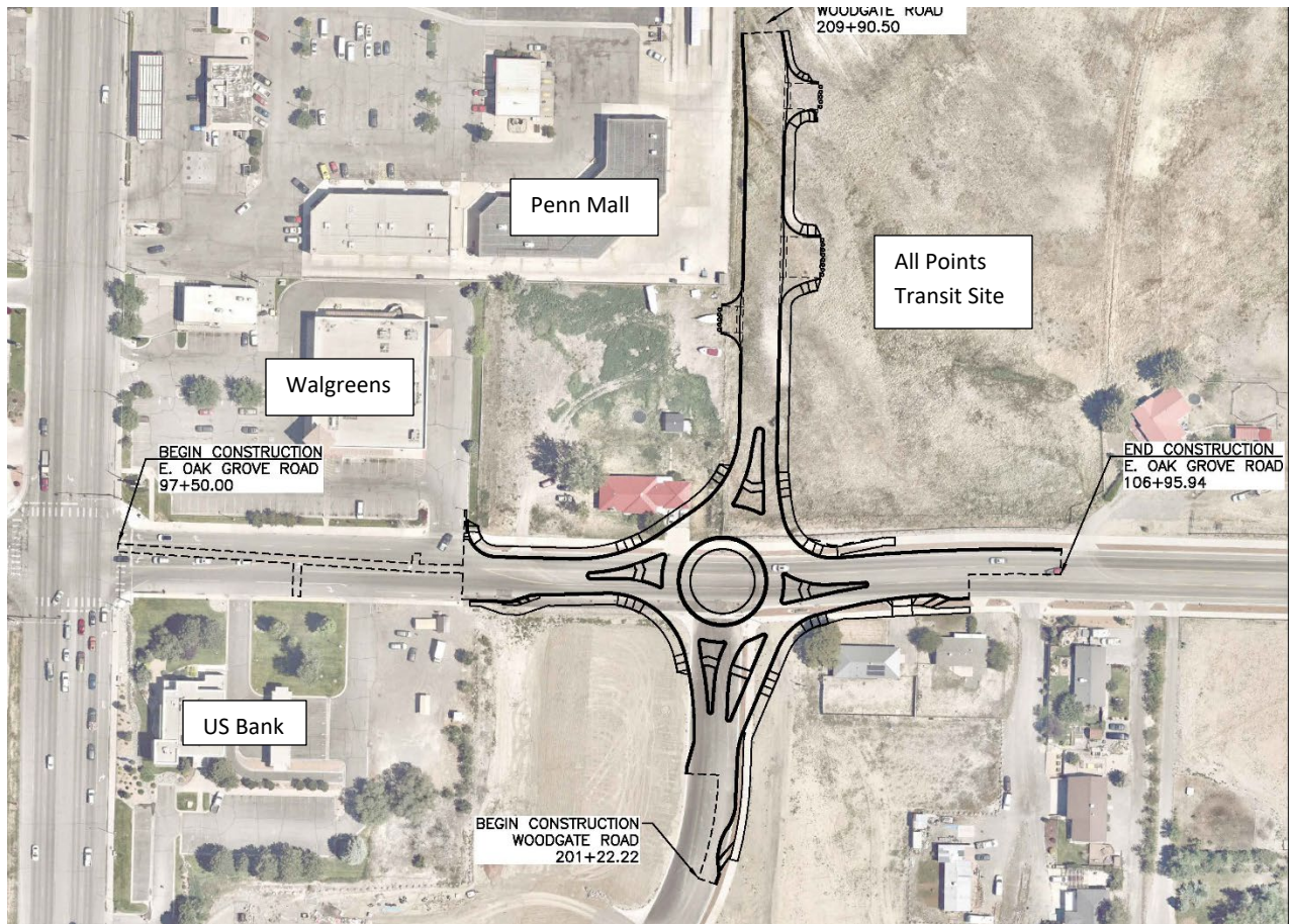
Figure 1: Project Overview Drawing
